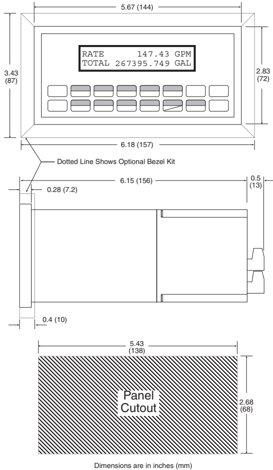
Fig. 1: Standard Dimensions
