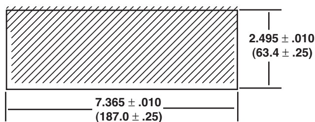
Panel Cutout
